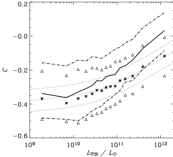
Figure 1. Observed IRAS FIR colour distribution [ C \equiv \log(S_{60}/S_{100}) ] as a function of 3–1100 \mu\text{m} TIR luminosity. Stars and triangles show the mean and 68 per cent confidence intervals when C is calculated from broad-band IRAS fluxes following the prescription in C03. The dotted lines show the mean and 1\sigma envelope of the fitted C03 colour–luminosity correlation for reference. The thick solid and dot-dashed lines show the mean and 68 per cent confidence intervals of the distribution when C is calculated with monochromatic flux densities emitted at 60 and 100 \mu\text{m} in the rest-frame.
