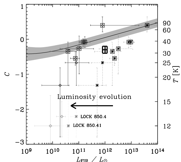
Figure 7. Comparison of local p(C|L) (shaded region is the 68 per cent confidence interval, solid line is C_0 from equation 9) with data from Coppin et al. (2008). The temperature axis is derived from C assuming a dust emissivity index \beta = 1.5 . Stars with dotted 1\sigma error bars indicate the 10 SMGs with spectroscopic redshifts and temperatures derived from observed 350/850\ \mu\text{m} colours. Squares have been drawn around the symbols for the six objects at z > 2 . High-redshift ultra-luminous galaxies appear systematically cooler than those in the local universe. Under the assumption of pure luminosity evolution of the form (1+z)^3 , the SMGs have been projected into the local colour–luminosity distribution by shifting them along the luminosity axis (diamonds with solid error bars). The model is a plausible fit to the data except for LOCK 850.4 and LOCK 850.41 which appear much cooler (shown as lighter symbols). These objects may have ambiguous or incorrect optical/IR counterpart identifications (discussed in Section 4.2). Future BLAST and SPIRE surveys will constrain FIR luminosities of \sim 10^{12} L_\odot galaxies to \sim 20 per cent, with uncertainties in C of \sim 0.1 (several Kelvin). A representative measurement in the L – C plane is given by the thick cross-filled square.
