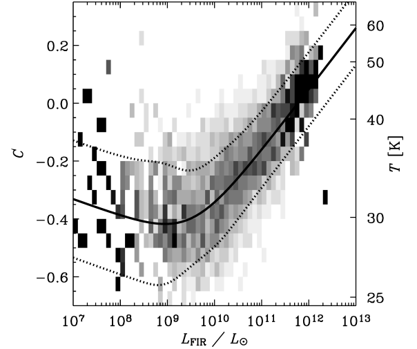
Figure 4. Comparison between parametric (solid and dotted lines give the mean and 1\sigma envelope of equation (8), respectively) and non-parametric estimates of p(C|L) (grey-scale shows \Phi_b(L, C) normalized along the C axis). The temperature axis is derived from C assuming a dust emissivity index \beta = 1.5 . At luminosities L \lesssim 10^8 and L \gtrsim 10^{12} , the sample does not contain enough galaxies to accurately constrain the shape, and p(C, L) is simply extrapolated in the parametric model.
