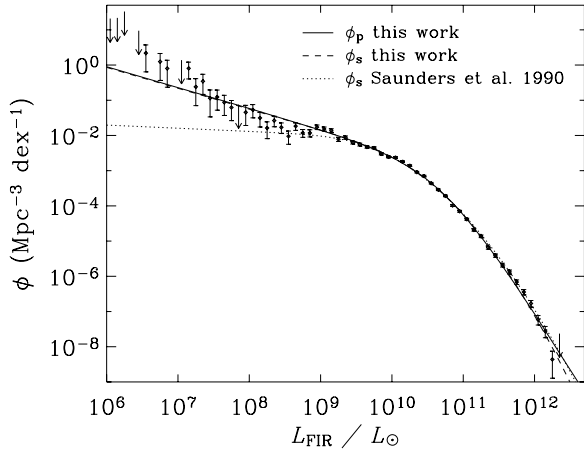
Figure 2. The non-parametric 42.5–122.5 \mu\text{m} FIR luminosity function (symbols with 68 per cent Poisson error bars and arrows show 95 per cent upper limits for bins with <2 objects) and two parametric fits (equation 6 as a solid line and equation 7 as a dashed line) derived from the S_{60} > 1.2 Jy IRAS sample of Fisher et al. (1995). The parametric FIR luminosity function of Saunders et al. (1990) is shown for comparison as a dotted line.
