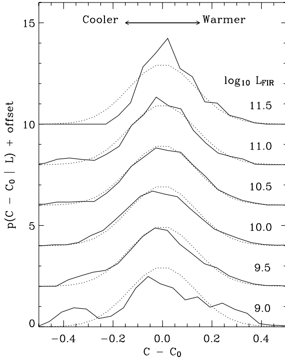
Figure 5. The distribution of FIR colours, C , about the mean, C_0 (equation 9), at a range of luminosities. The solid lines are normalized slices of the measured (non-parametric) p(C|L) [ \Phi_b(L, C)/\Phi_b(L) – see equations 1 and 5] evaluated at C - C_0 , and numbers indicate \log_{10} L_{\text{FIR}} . The parametric model (equation 8) is shown as a dotted line.
