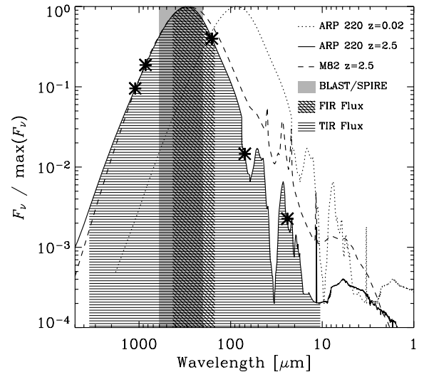
Figure 6. The peak-normalized SED of Arp 220 (dotted line) and shifted to z = 2.5 (solid line). The complete observed BLAST and SPIRE band (200–600 \mu\text{m} , including the 30 per cent finite bandpasses for each channel) is indicated by the solid grey-shaded rectangle. The rest-frame 3–1100 \mu\text{m} TIR flux and 42.5–122.5 \mu\text{m} FIR flux correspond to the integrals of the horizontal-line filled and cross-hatch filled regions, respectively, for the z = 2.5 SED. Clearly for objects at this redshift, the BLAST and SPIRE filters match the rest-frame FIR flux more closely than the TIR flux. The peak-normalized M82 SED redshifted to z = 2.5 (shown as a dashed line) illustrates the relatively large variations in the rest-frame MIR spectrum ( \sim 3 – 60 \mu\text{m} observed wavelength). Symbols indicate the wavelengths accessible from ground-based submillimetre surveys (e.g. SCUBA at 850 \mu\text{m} and AzTEC/MAMBO at 1.1 mm), and existing space-based FIR data (e.g. Spitzer at 24, 70 and 160 \mu\text{m} ), demonstrating their inability to accurately constrain the bolometric FIR luminosity for these galaxies.
