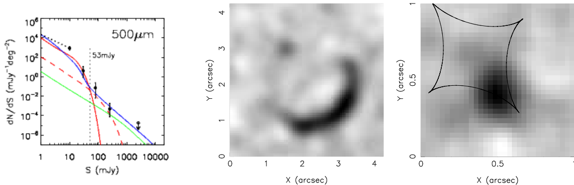
FIG. 10.— The left-hand panel shows the predicted number of sources as a function of 500\mu\text{m} flux density plotted over the results from BLAST (Negrello et al. 2007). The key to the curves is as follows: red solid—unlensed high- z protospheroids; red dashed—lensed high- z protospheroids; green—blazars; blue—nearby late-type galaxies. The vertical dashed line shows the approximate limit of H-ATLAS at 500\mu\text{m} . The middle panel shows a simulated image of a strongly lensed 100\text{mJy} 500\mu\text{m} H-ATLAS source as observed using the Submillimetre Array at 870\mu\text{m} in extended mode over a 6h track. The panel on the right shows the reconstructed source obtained by applying the reconstruction method of Dye et al. (2007a) to the simulated ring image. The image caustic of the best fit lens model is over-plotted.
