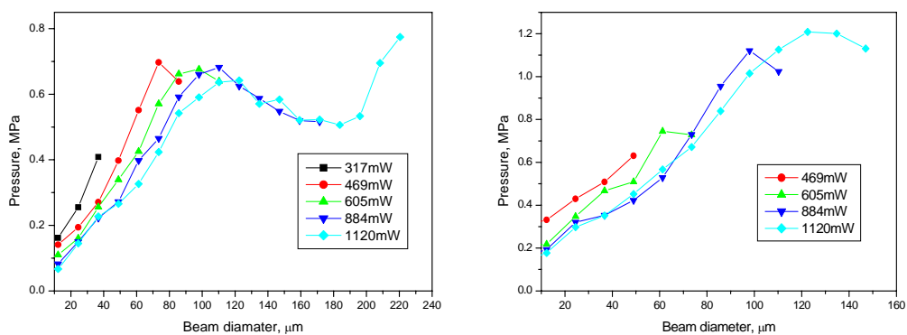
Figure 2. Shock wave pressure as function of the input beam diameter for different incident light power and liquid absorption coefficients 90 \text{ cm}^{-1} (left) and 45 \text{ cm}^{-1} (right). Permanent illumination, every point represents an average over 200 collapse events.
