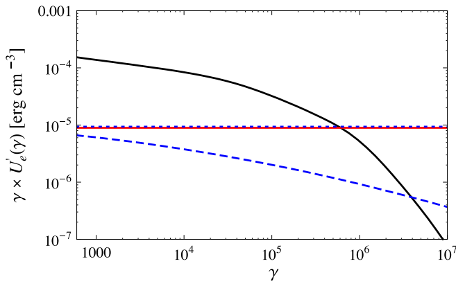
Figure 11. Jet comoving energy density of ultrarelativistic electrons per logarithmic energy bin, \gamma U'_e(\gamma) , as a function of the electron Lorentz factor \gamma (solid black curve). For comparison, the comoving energy density of the magnetic field U'_B (solid red line) and synchrotron photons U'_{syn} (dotted blue line) are shown. The dashed blue curve denotes the comoving energy density of synchrotron photons which are inverse-Compton upscattered in the Thomson regime, U'_{syn/T} , for a given electron Lorentz factor \gamma (see equation 12).
