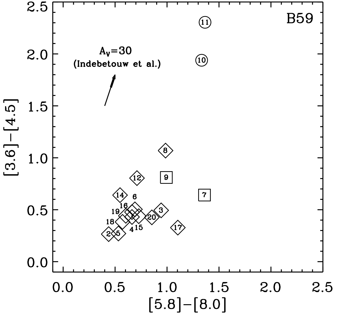
Fig. 6.— IRAC color-color diagram, as observed, of candidate young stars in B59 with source numbers from Table 1. Young star IR spectral classes, after correction for extinction (where possible) are indicated with the following symbols: Class I ( circle ), Flat ( square ), and Class II ( diamond ). The reddening arrow shows the adopted extinction law (Indebetouw et al., 2005) for A_V \approx 30 mags (see text).
