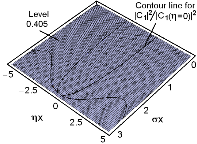
Figure 4. A 2D-contour for the normalized light intensity on the plane [(\sigma x), (\eta x)] on the interval 0 \leq \sigma x \leq \pi .
