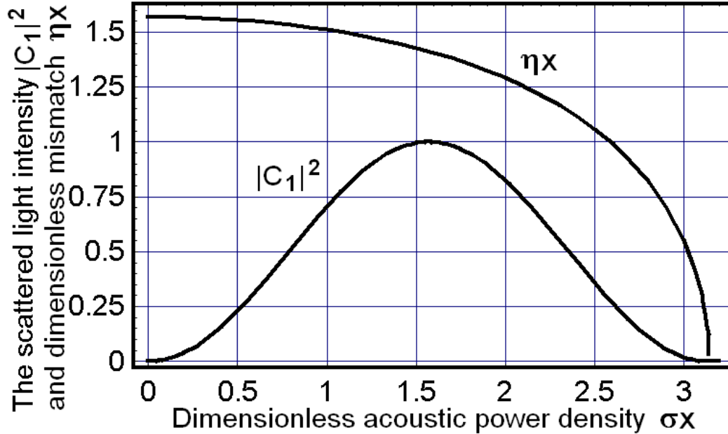
Figure 3. The light intensity |C_1(x)|^2 and a one-side dimensionless mismatch \eta x versus the product \sigma x .
