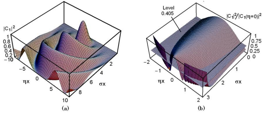
Figure 1. The 3D-plots of the scattered light intensity profile with q_0/q_1 \approx 1 : (a) for the absolute values on the interval 0 \leq \sigma x < 3\pi and (b) for the normalized distribution on the interval 0 \leq \sigma x \leq \pi .
