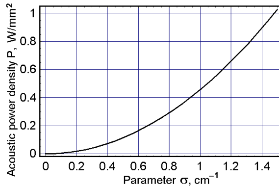
Figure 7. Acoustic power density P vs. the parameter \sigma at \lambda = 671 \text{ nm} in the above-chosen collinear \text{CaMoO}_4 -crystalline cell.
