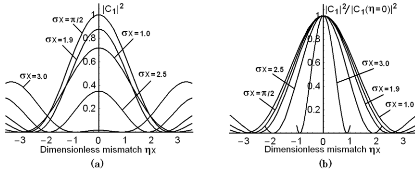
Figure 2. The 2D-plots |C_1[(\sigma x), (\eta x)]|^2 for the products 1.0 \leq \sigma x < \pi with q_0/q_1 \approx 1 : (a) for the absolute values and (b) after normalization by the zero magnitudes.
