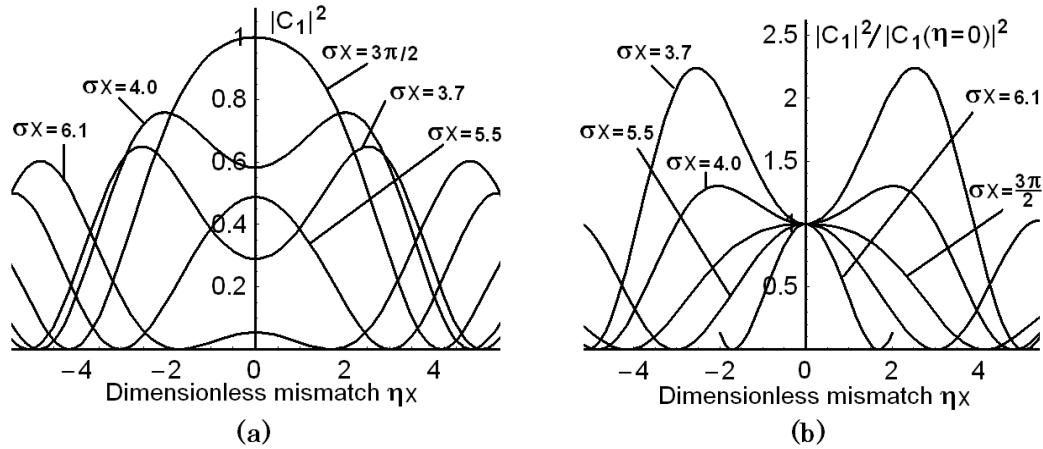
Figure 5. The 2D-plots |C_1[(\sigma x), (\eta x)]|^2 for the products \pi < \sigma x < 2\pi with q_0/q_1 \approx 1 : (a) for the absolute values and (b) after normalization by the zero magnitudes.
