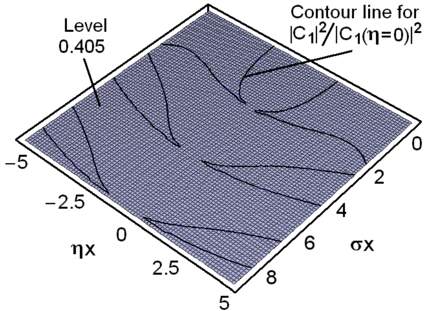
Figure 6. A 2D-contour plot for the normalized light intensity on the plane [(\sigma x), (\eta x)] on the interval 0 \leq \sigma x < 3\pi .
