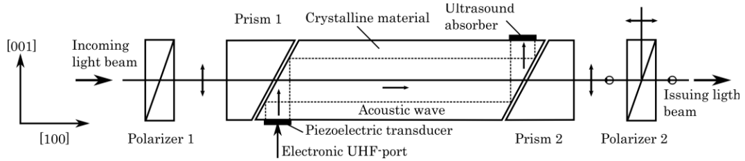
Figure 9. Scheme of the co-propagating collinear \text{CaMoO}_4 -cell providing the traveling-wave regime of interaction between the pumping light beam and the continuous-wave lossless acoustic beam.
