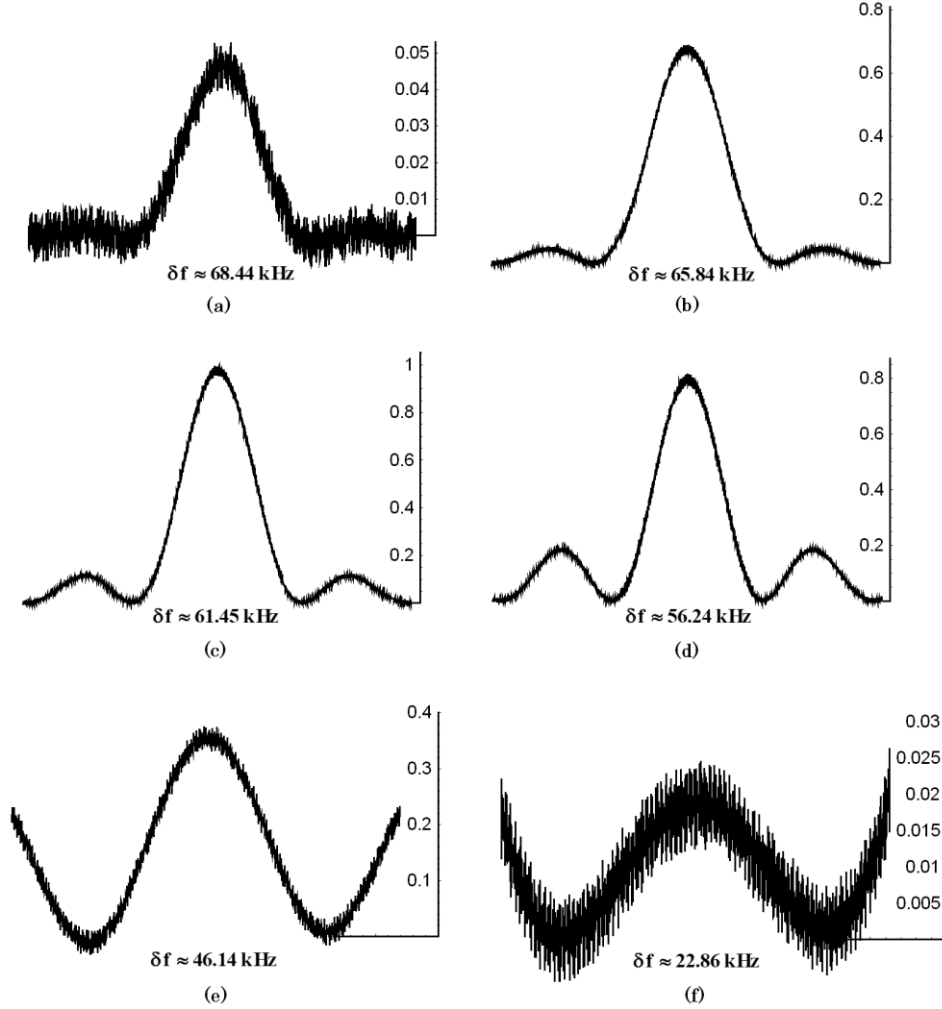
Figure 10. The digitized oscilloscope traces for the scattered light intensity |C_1|^2 observed at the output of the collinear \text{CaMoO}_4 cell at the carrier acoustic frequency of \sim 37.3 MHz and estimated at the level 0.405. Reshaping the transmission function is followed at the same optical pump in variable scales:
