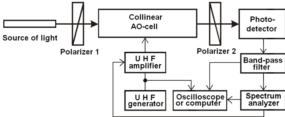
Figure 8. Schematic arrangement of the experimental set-up
