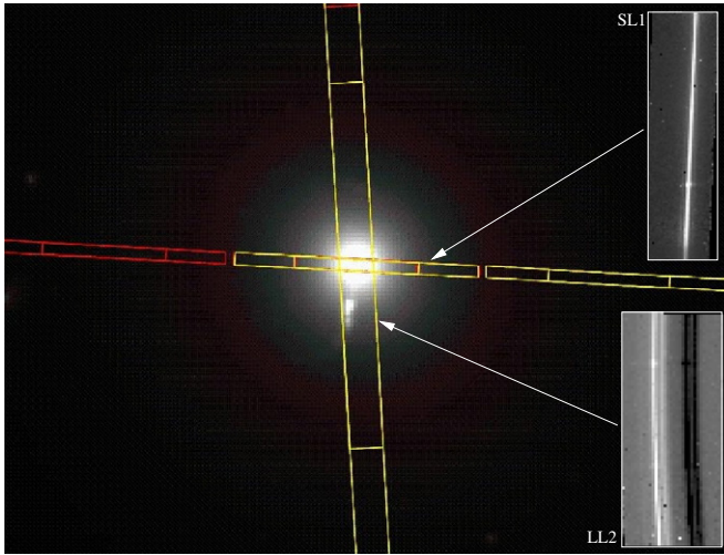
Figure 1. IRS SL (nearly horizontal) and LL (nearly vertical) slits superimposed on the MIPS image of M 87 at \lambda = 24 \mu\text{m} . The two additional panels on the right side show a portion of the LL2 (bottom) and SL1 (top) two-dimensional spectral images. Note that the former does clearly show both the spectra of the nucleus and that of the nearest bright knots, whereas the SL slit is not affected by these components. The extraction width of the LL spectra does not include the contribution from these knots.
