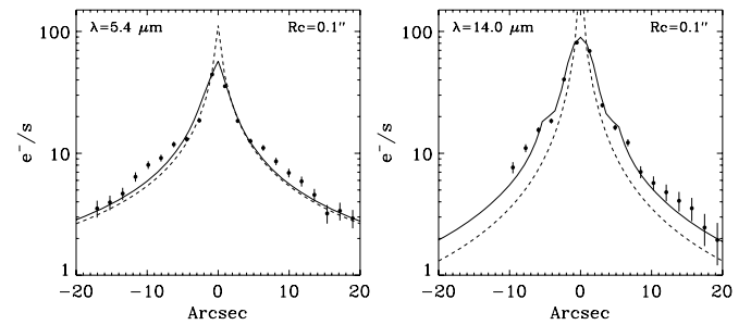
Figure 2. NGC 4486 spatial emission profiles (filled dots), in electrons \text{s}^{-1} , at two selected wavelengths. The dashed lines show the reconstructed one-dimensional intrinsic spatial emission profiles sampled along the slit, while the solid lines represent the corresponding one-dimensional PSF convolved models that are fitted to the data. Error bars are 1\sigma uncertainties.
