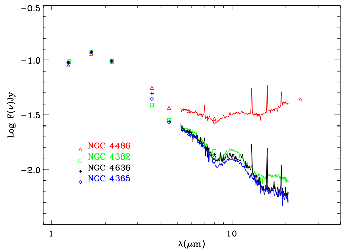
Figure 3. NIR/MIR SED of M 87 (NGC 4486) and of the other three passive galaxies in a circular aperture of 4'' radius. The passive ETGs have been normalized to the K_s broadband flux of M 87.
