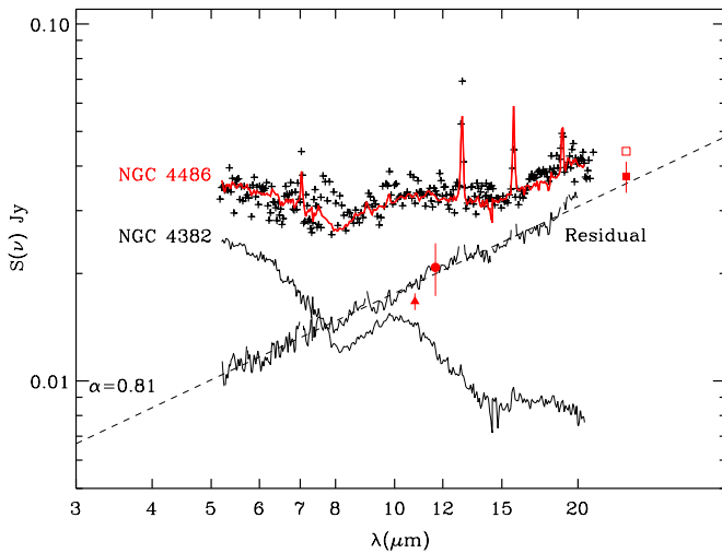
Figure 4. MIR residual after subtracting the K_s band-normalized template SED of NGC 4382 from that of M 87 (NGC 4486), both indicated in the figure. The exponent of the power-law fit (dashed line, S_\nu \propto \nu^{-\alpha} ) is shown. The dot and triangle mark the 11.67 \mu\text{m} and 10.8 \mu\text{m} ground-based nuclear measurements by Perlman et al. (2007) and Perlman et al. (2001), respectively. The open square is the M 87 MIPS 24 \mu\text{m} flux. After correction for the NGC 4382 extrapolated emission, the M 87 MIPS 24 \mu\text{m} flux lowers to the position indicated by the filled square. Crosses show another IRS spectrum of M 87 that was extracted from the archive data (ID 82, PI: G. H. Rieke) used by Perlman et al. (2007). (A color version of this figure is available in the online journal.)
