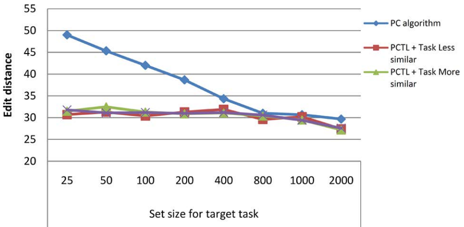
Fig. 12 Behavior of the proposed method (PC-TL) as the number of samples of the target task increases (Insurance network)
