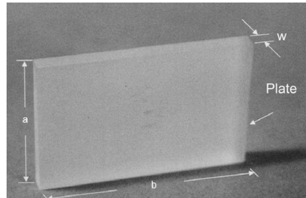
Fig. 3. Real glass plate showing the dimensions and the width w of the plate in the laboratory.
