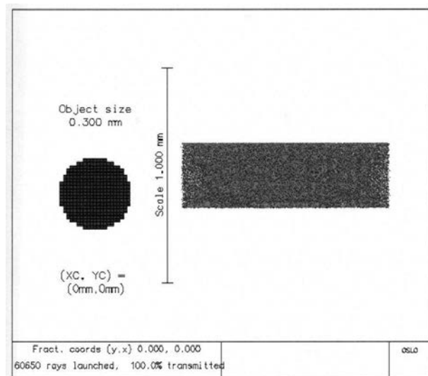
Fig. 7. Ray trace of the system for a round entrance image that produces the illuminated strip on the back side of the plate.
