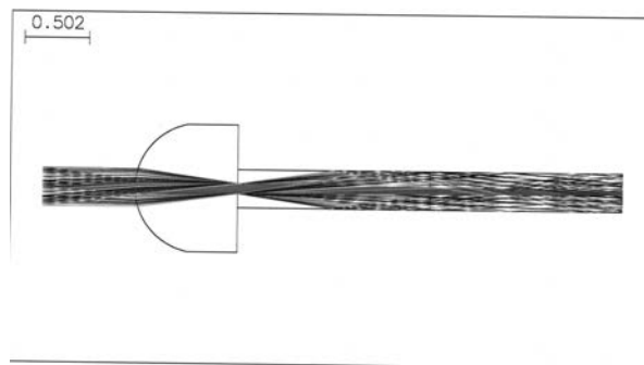
Fig. 5. Meridional ray trace of the transformer showing the waist of the beam and the internal reflections.
