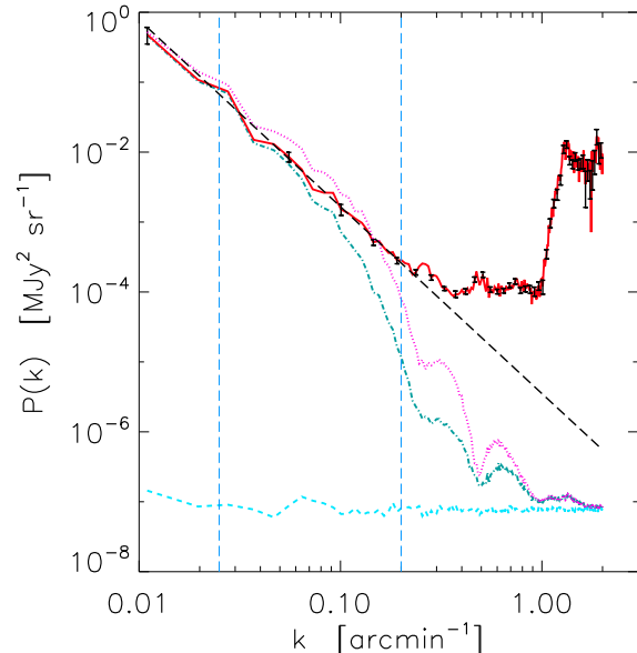
FIG. 2.— BLAST power spectra at 250 \mu\text{m} for the Cyg X region shown in Fig. 4. The dotted curve, corresponding to the upper panel of Fig. 4, shows that a significant amount of power is present at intermediate scales due to compact sources. The lower dot-dash line is P(k) of the same region after removing sources (corresponding to Fig. 5). The oscillatory behavior at large k is due to the corrupted BLAST05 PSF (Fig. 3). The almost horizontal dashed line is the power spectrum of the noise map (§ 5.1). At very small scales where the astronomical signals become correlated within the beam, the power spectra meet the noise level. The solid line is the power spectrum P_{\text{cirrus}}(k) , after subtracting the noise and dividing by \Gamma(k) to remove the effect of the beam (as in Fig. 1, error bars at high k do not include the imperfect knowledge of the beam and noise). The vertical dashed lines indicate the restricted range 0.025 \text{ arcmin}^{-1} < k < 0.2 \text{ arcmin}^{-1} used for fitting the power law. The exponent is -2.60 \pm 0.07 and P(0.1 \text{ arcmin}^{-1}) = (1.60 \pm 0.05) \times 10^{-3} \text{ MJy}^2 \text{ sr}^{-1} .
