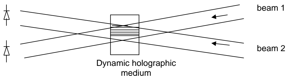
Figure 1. The principle of adaptive interferometry. Two beams write a hologram in a medium and diffract on it. The photodetector pair detects rapid phase shifts, which are not compensated by a medium.
