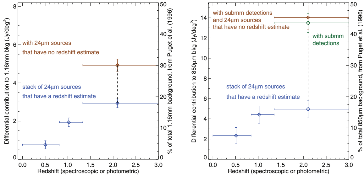
Figure 9. Left-hand panel: the (differential) redshift distribution of the resolved 1.16 mm background from 24 \mu\text{m} sources. The diamonds are plotted at the average redshifts of the bins. The brown diamond contains the contributions from the 24 \mu\text{m} sources with z > 1.3 and the 24 \mu\text{m} sources without a redshift estimate. Right-hand panel: the (differential) redshift distribution of the resolved 850 \mu\text{m} background from 24 \mu\text{m} sources. We use the same redshift bins as in the left-hand panel. The y-axes in both panels show the levels at which the backgrounds are 50 per cent resolved. Most of the resolved background at the two wavelengths comes from galaxies at z > 1.3 .
