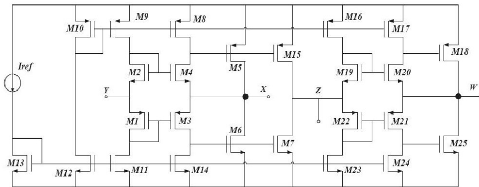
Figure 4. Current-Feedback Operational Amplifier (CFOA).
