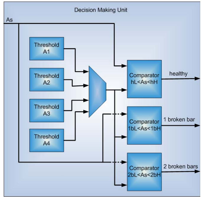
Fig. 5. Decision-making unit.
