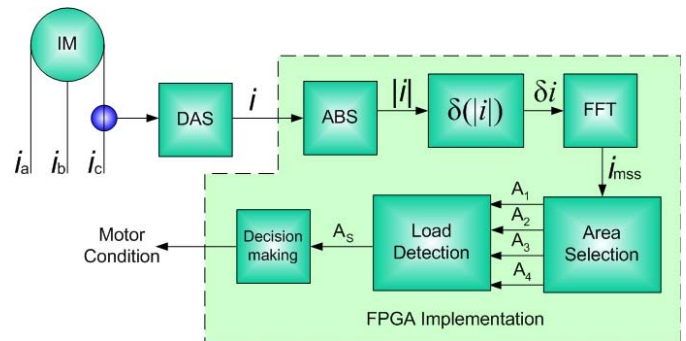
Fig. 3. Proposed methodology.
