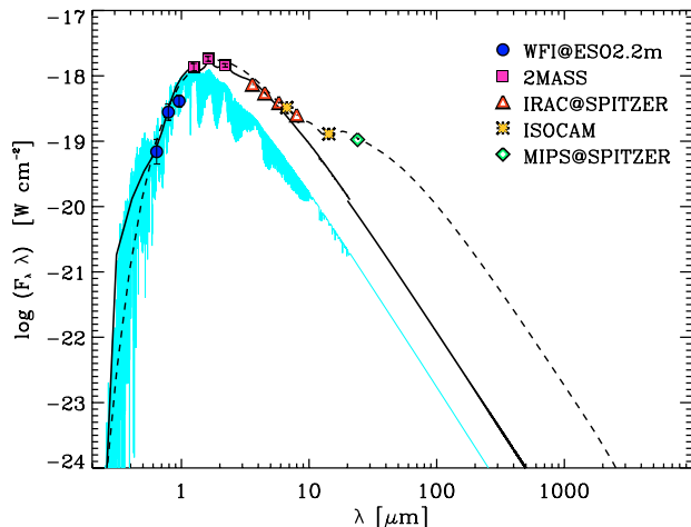
Fig. 3. Spectral energy distribution of ISO-CHA II 13. The StarDusty spectrum with the same temperature as the BD is over-plotted. The continuous line is the sum of the star and disk emissions assuming black-body emission from the disk, while the dashed line is the result of the fit performed with the FitCGplus tool by Dullemond et al. (2001).
